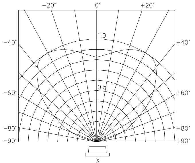
Radiation Diagram
